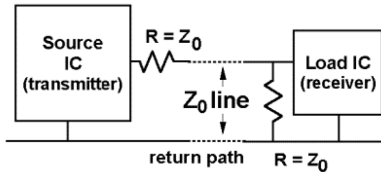
Figure 2G Transmission line terminations
