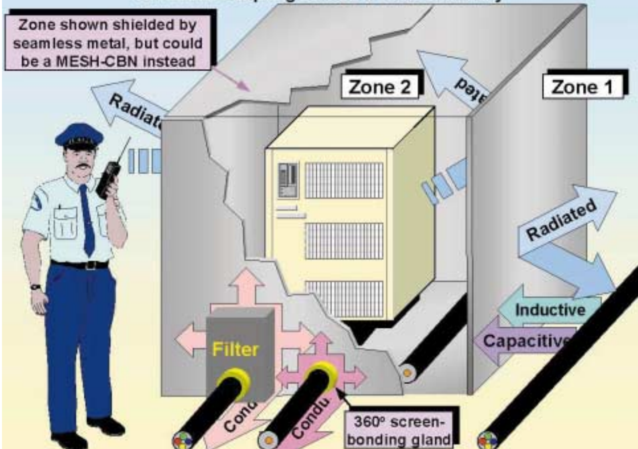
Figure 4D Using filtering and shielding to reduce coupling across a zone boundary
