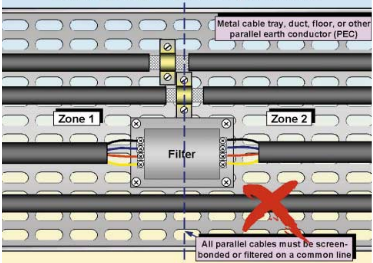
Figure 4F Filtering or screen-bonding parallel cables
