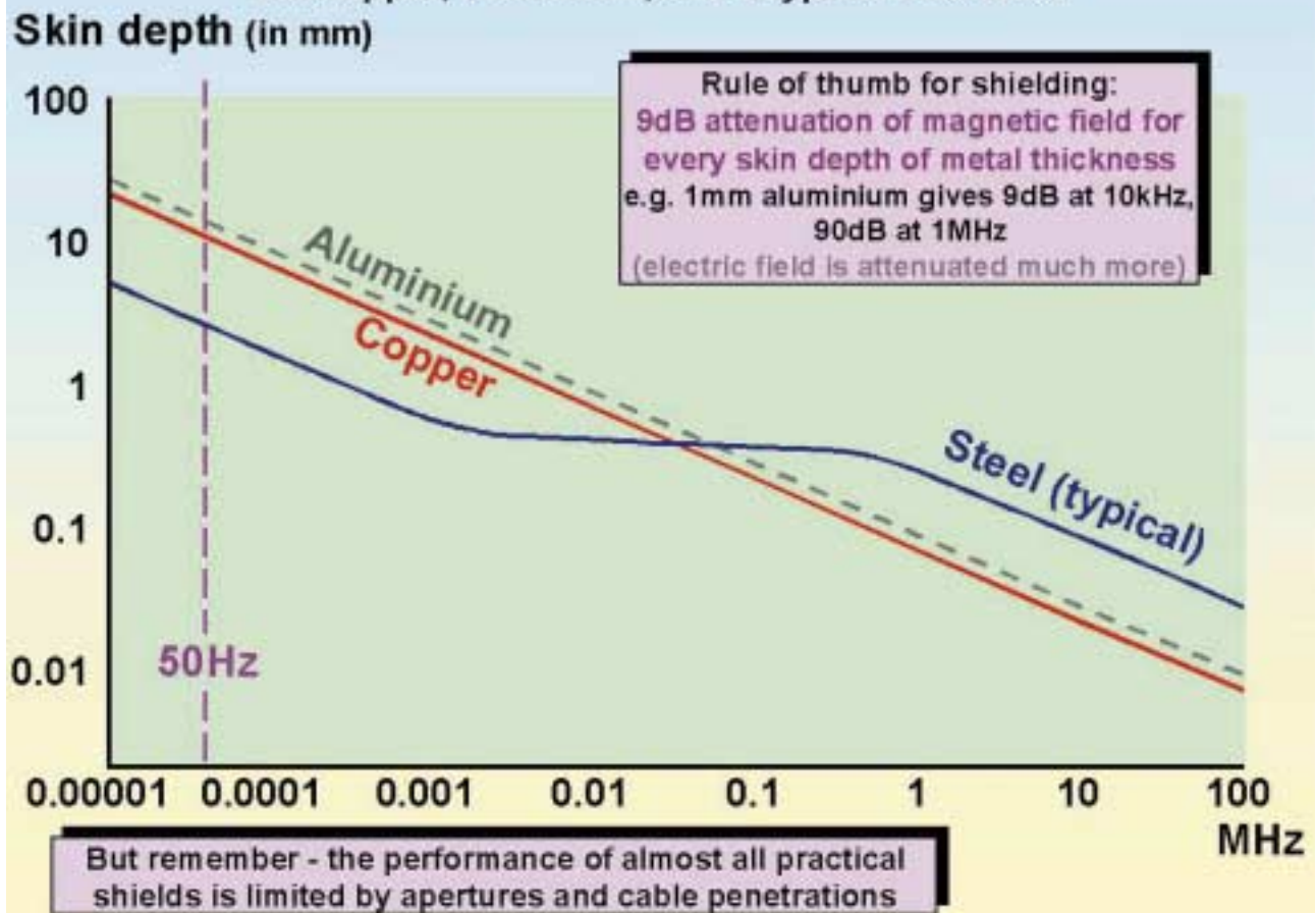
Figure 4G Graph of skin depths for copper, aluminium, and a typical mild steel
